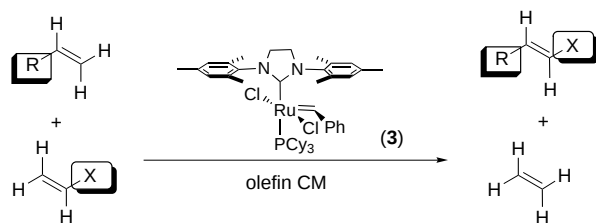
Scheme 1. Direct cross-coupling of olefins.
